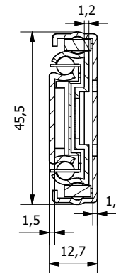
C-C (1:1)
