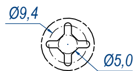
B (1:1)
