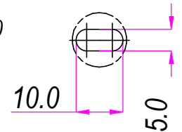
(1:3) SEZ AA'
