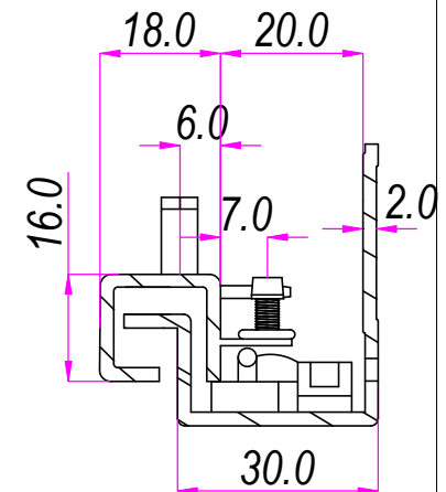
(1:3) SEZ AA'
