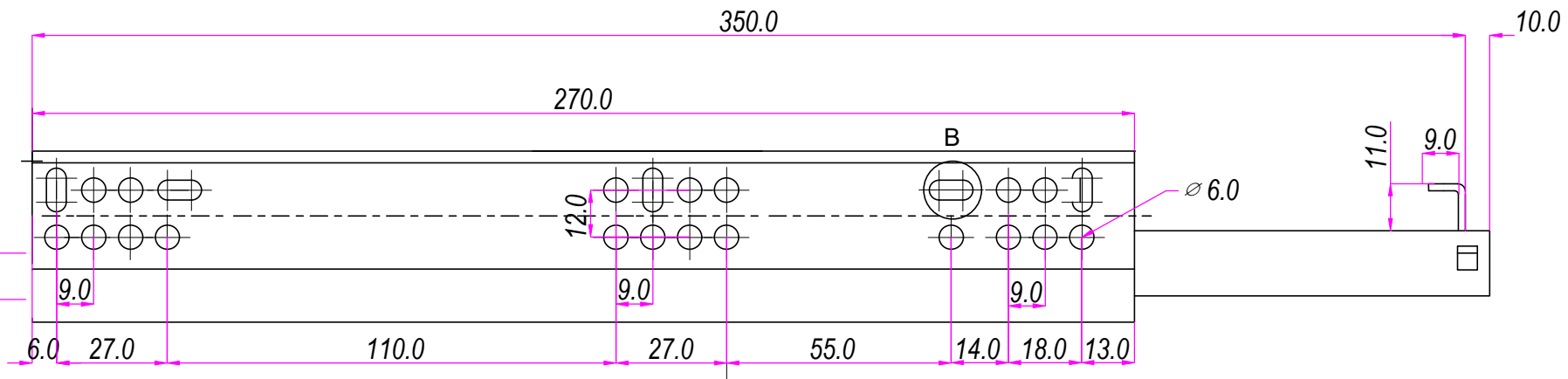
(1:3) SEZ AA'
