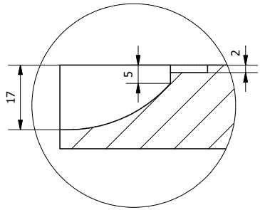
B (1:1)
